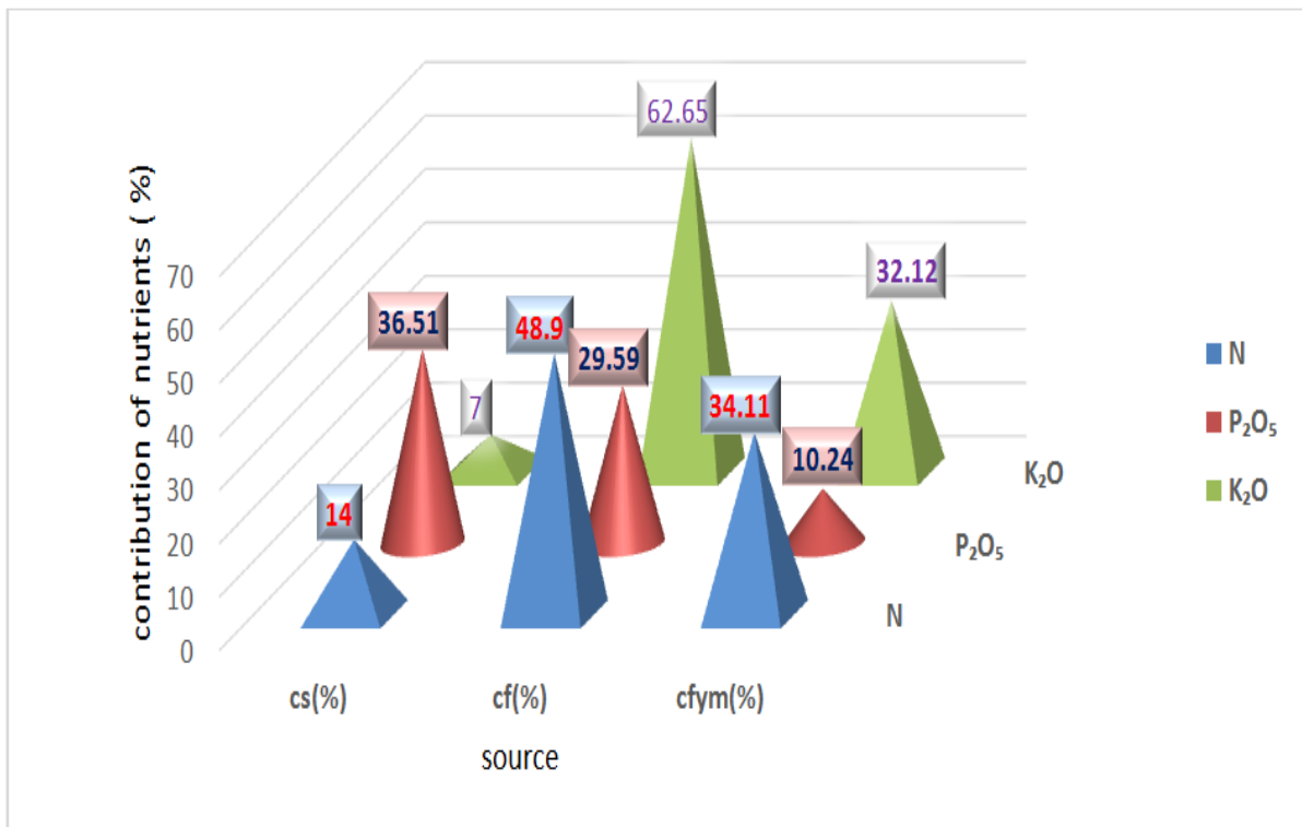
Fig. 2. Contribution of nutrients from soil (Cs %), fertilizer (Cf%) and (Cfym%)
