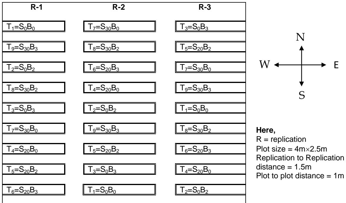
Fig. 2. Layout of the experimental field
