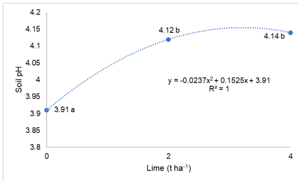
Fig. 1. A quadratic trend from orthogonal polynomial contrast for lime treatment to increase soil pH value. Means followed by the same letters are not significantly different at DMRT 5%
