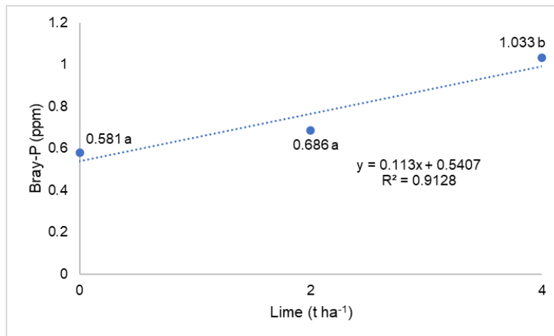
Fig. 3. A linear trend from orthogonal polynomial contrast for lime treatment on available-P. Means followed by the same letters are not significantly different at DMRT 5%
