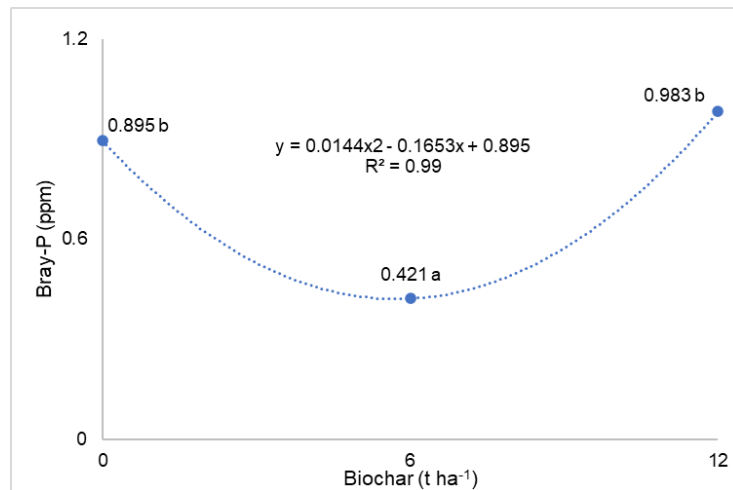
Fig. 2. A quadratic trend from orthogonal polynomial contrast for biochar treatment on available-P. Means followed by the same letters are not significantly different at DMRT 5%
