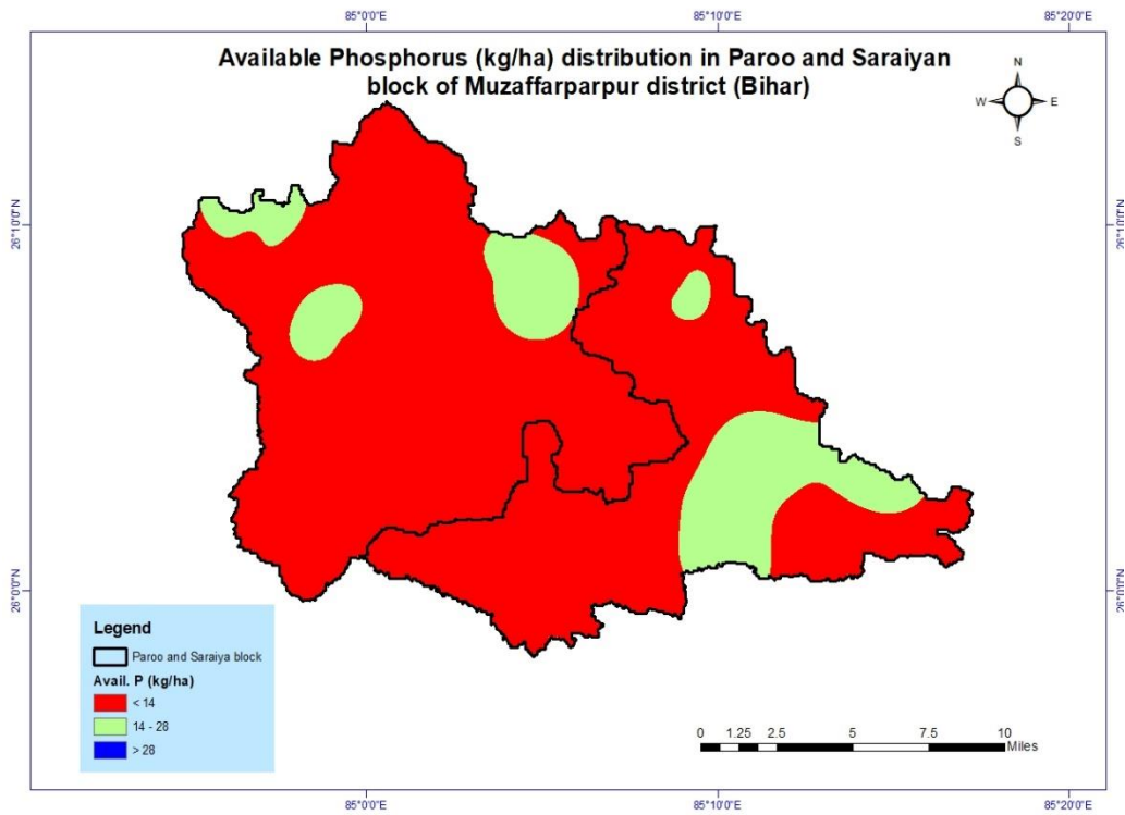
Fig. 6. Distribution of available Phosphorus ( \text{kg ha}^{-1} ) in Paroo and Saraiyan Block of Muzaffarpur district, Bihar
