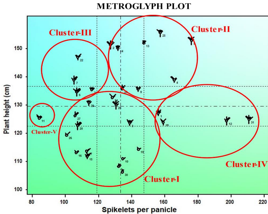
Fig. 2. Scattered diagram of Metroglyph analysis showing 31 genotypes of rice
