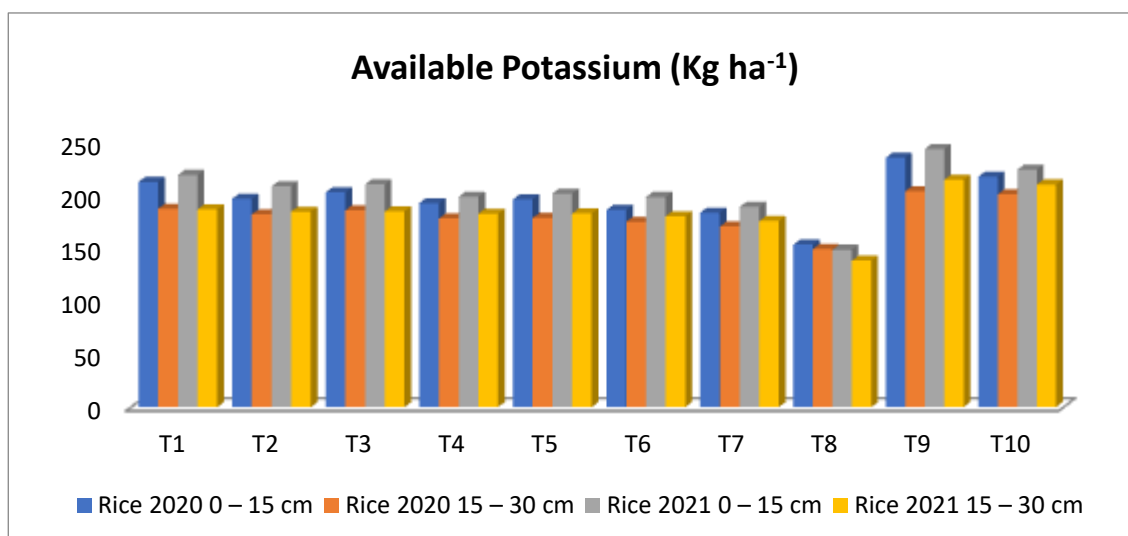
Fig. 6. Impact of crop residue and green manure on soil available potassium
