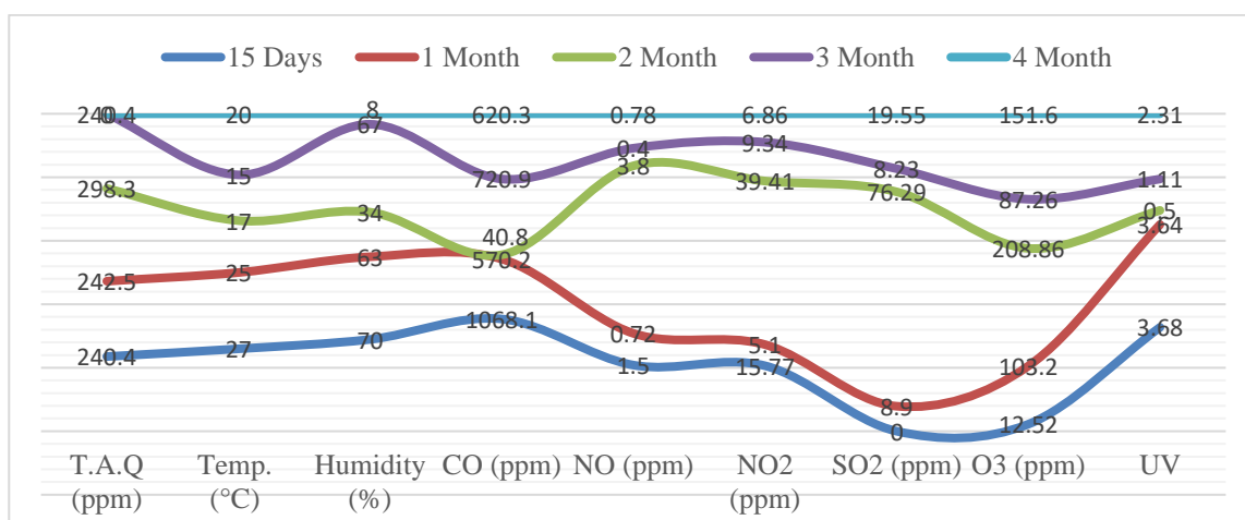
Fig. 2. Variable gas concentrations at the under-road traffic site
