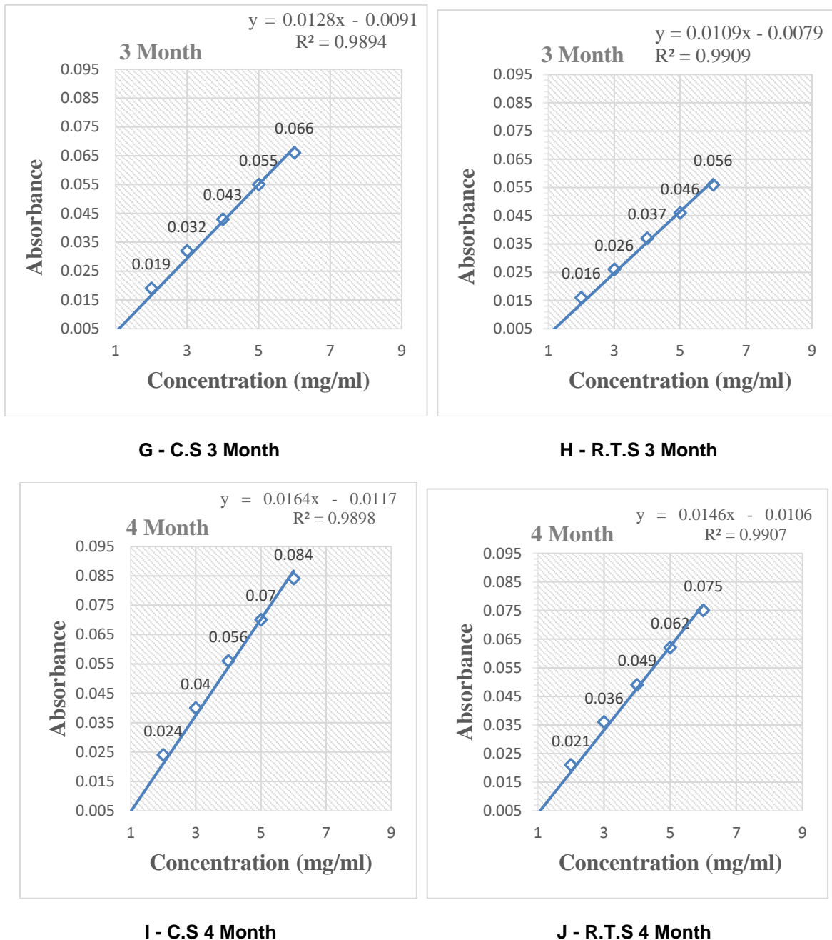
Fig. 3. The standard curve showing the total phenolic content value at various intervals under the control and road traffic sites C.S – Control Site; R.T.S – Road Traffic Site
