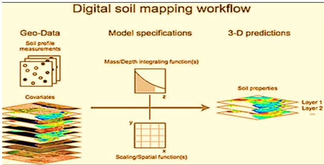
Fig. 5. Workflow of digital soil mapping
