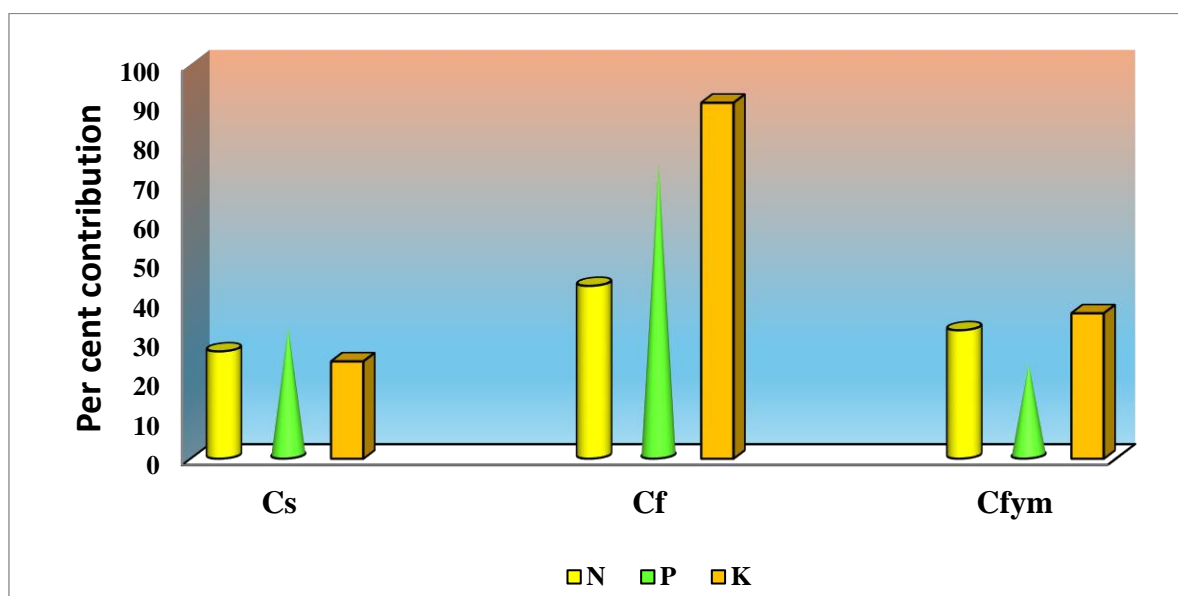
Fig. 4. Per cent contribution of nutrients from soil, fertilizer and FYM
