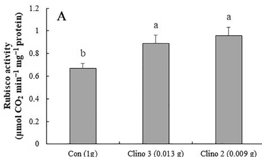
Fig. 7. Rubisco enzyme activity
