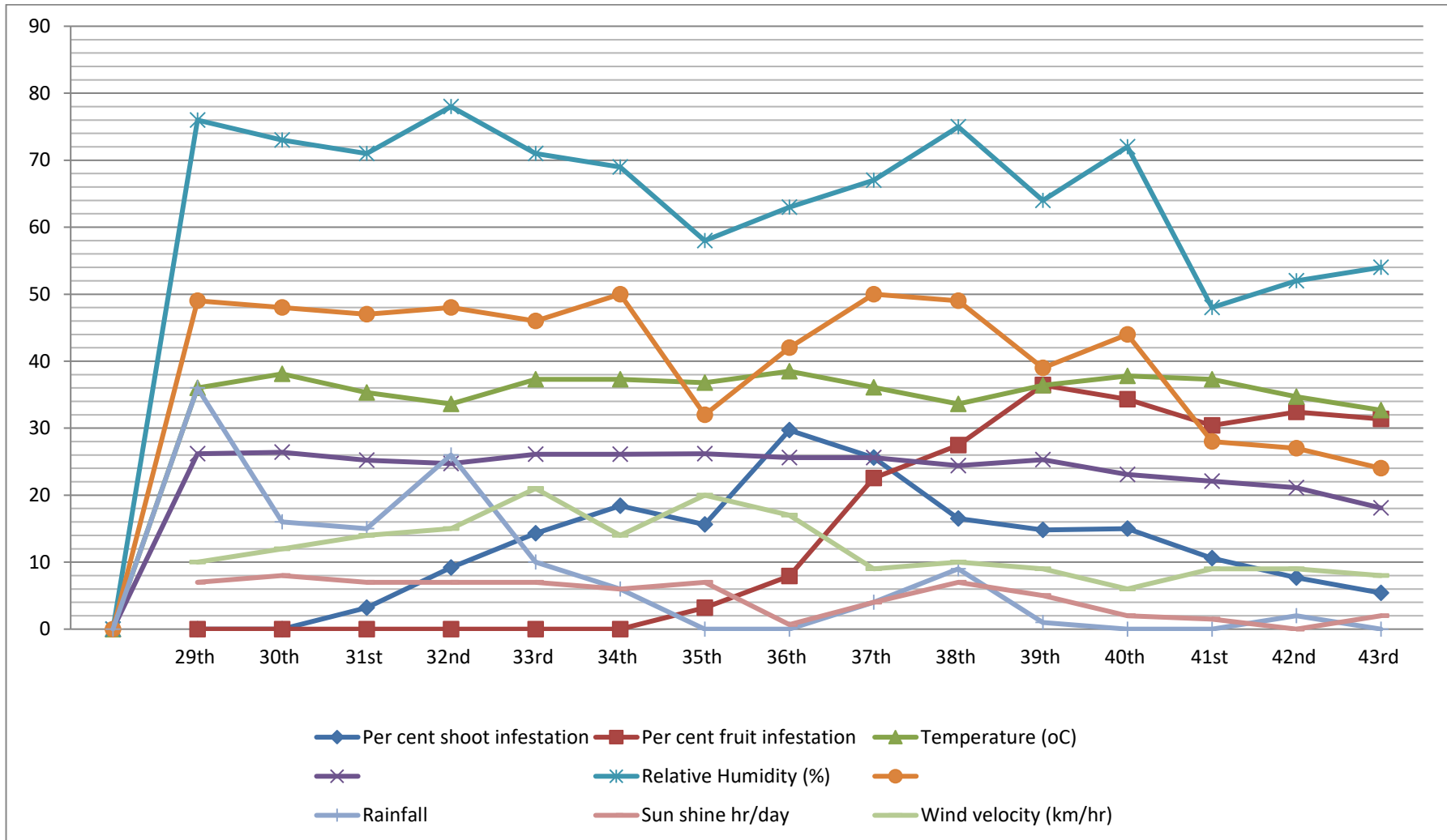
Fig. 1. Seasonal incidences of shoot and fruit borer ( Earias vittella ) on okra in relation to abiotic factor during kharif 2023
