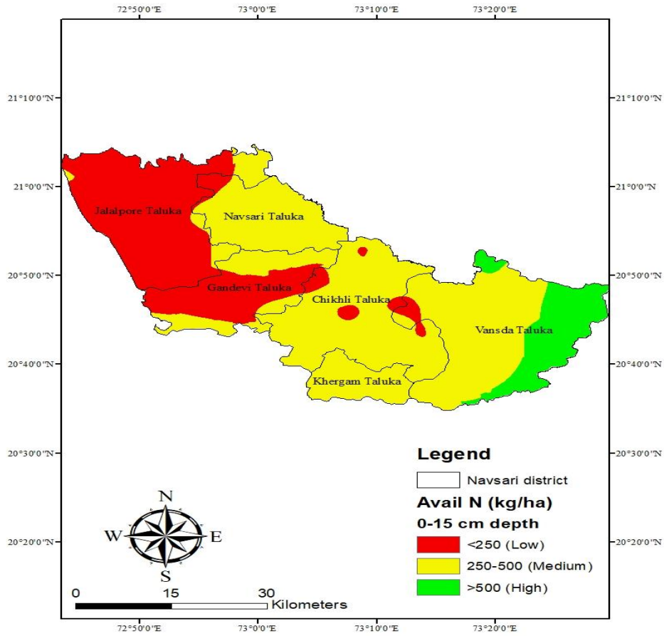
Fig. 2. Available Nitrogen(kg/ha) status at 0-15 cm depth
