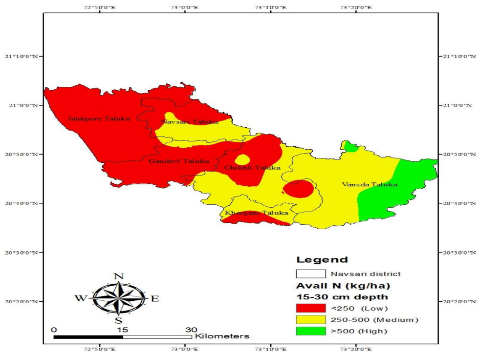
Fig. 3. Available Nitrogen (kg/ha) status at 15-30 cm depth
