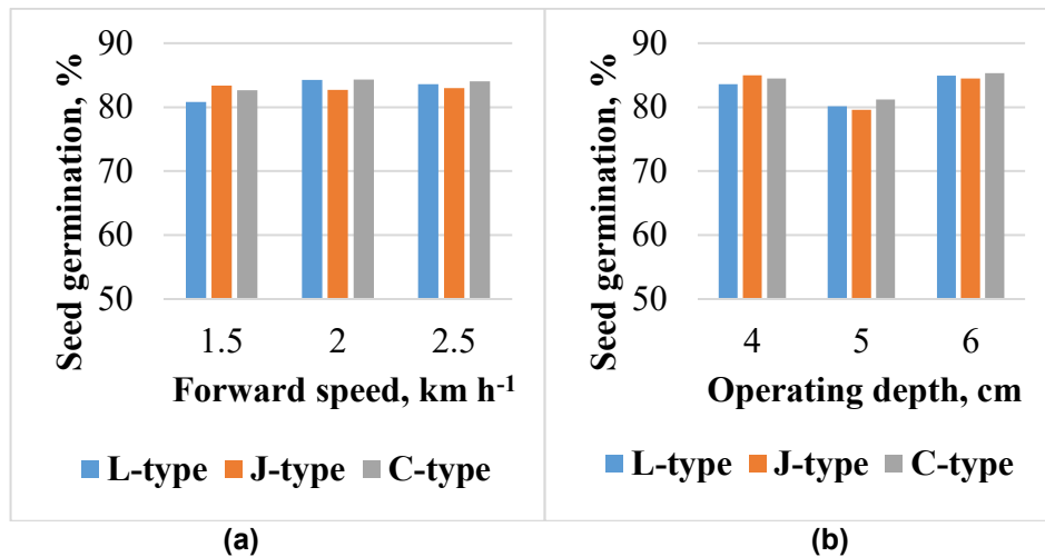
Fig. 5. Seed germination at different forward speed and operating depth for three types of rotary blades
