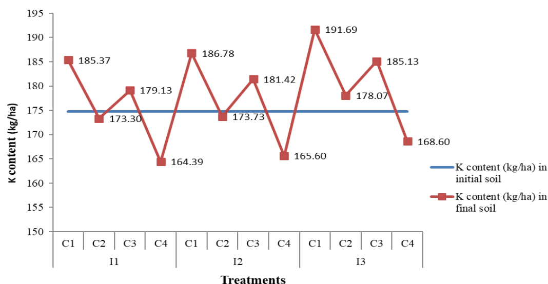
Fig. 3. Initial and final soil potassium (kg/ha)
