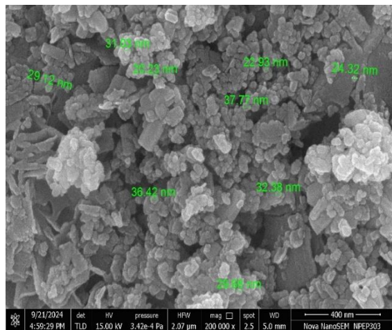
Fig. 1 (c). Characterization of nano zinc oxide (ZnO) particles for size using SEM
