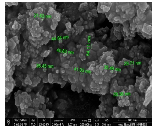
Fig. 1 (d). Characterization of nano zinc oxide (ZnO) particles for size using SEM
