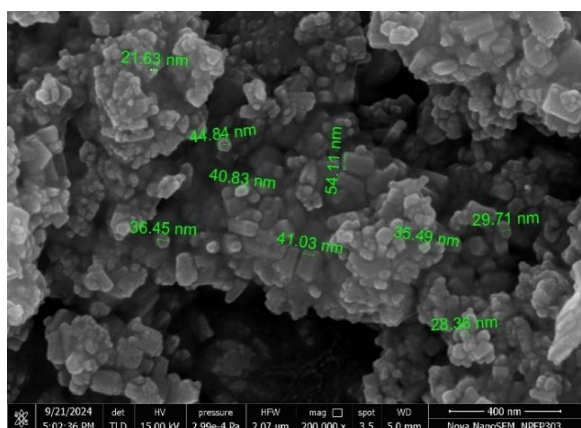
Fig. 1 (d). Characterization of nano zinc oxide (ZnO) particles for size using SEM
