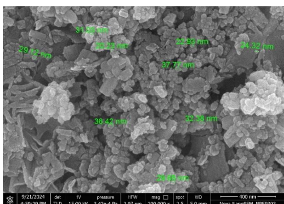
Fig. 1 (c). Characterization of nano zinc oxide (ZnO) particles for size using SEM
