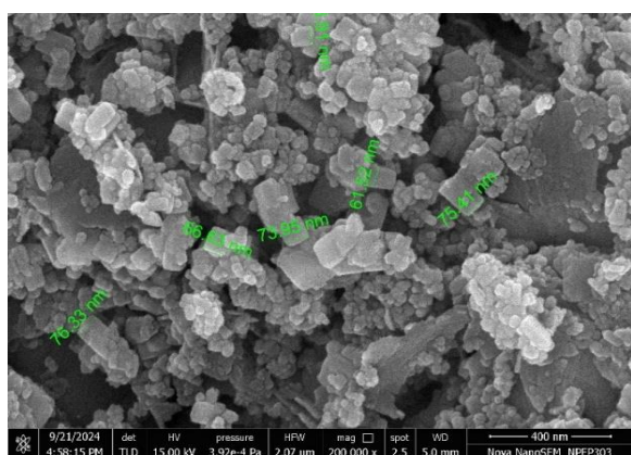
Fig. 1 (b). Characterization of nano zinc oxide (ZnO) particles for size using SEM
