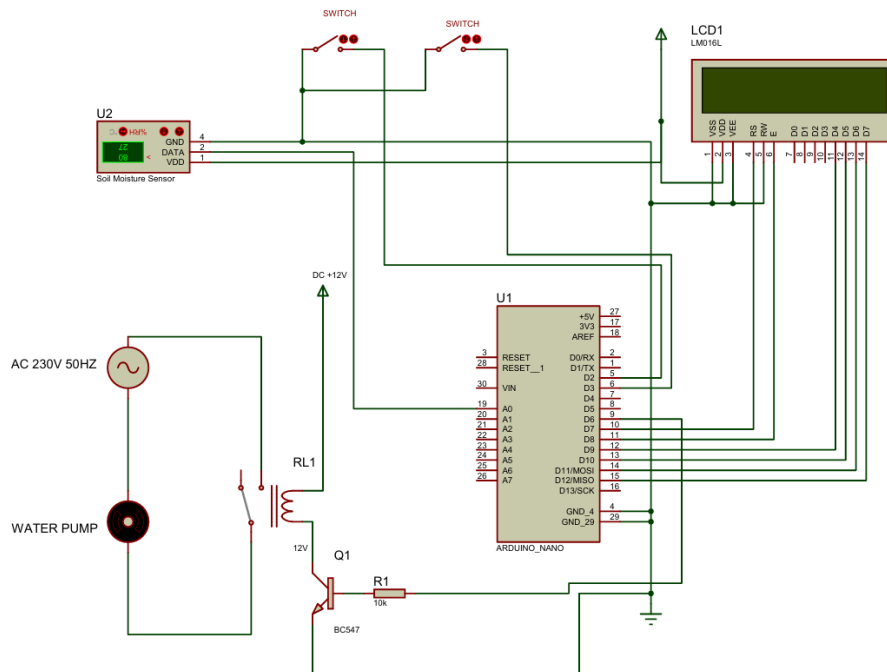
Fig. 1. Circuit Diagram of Crop-specific and soil-responsive automated irrigation system
