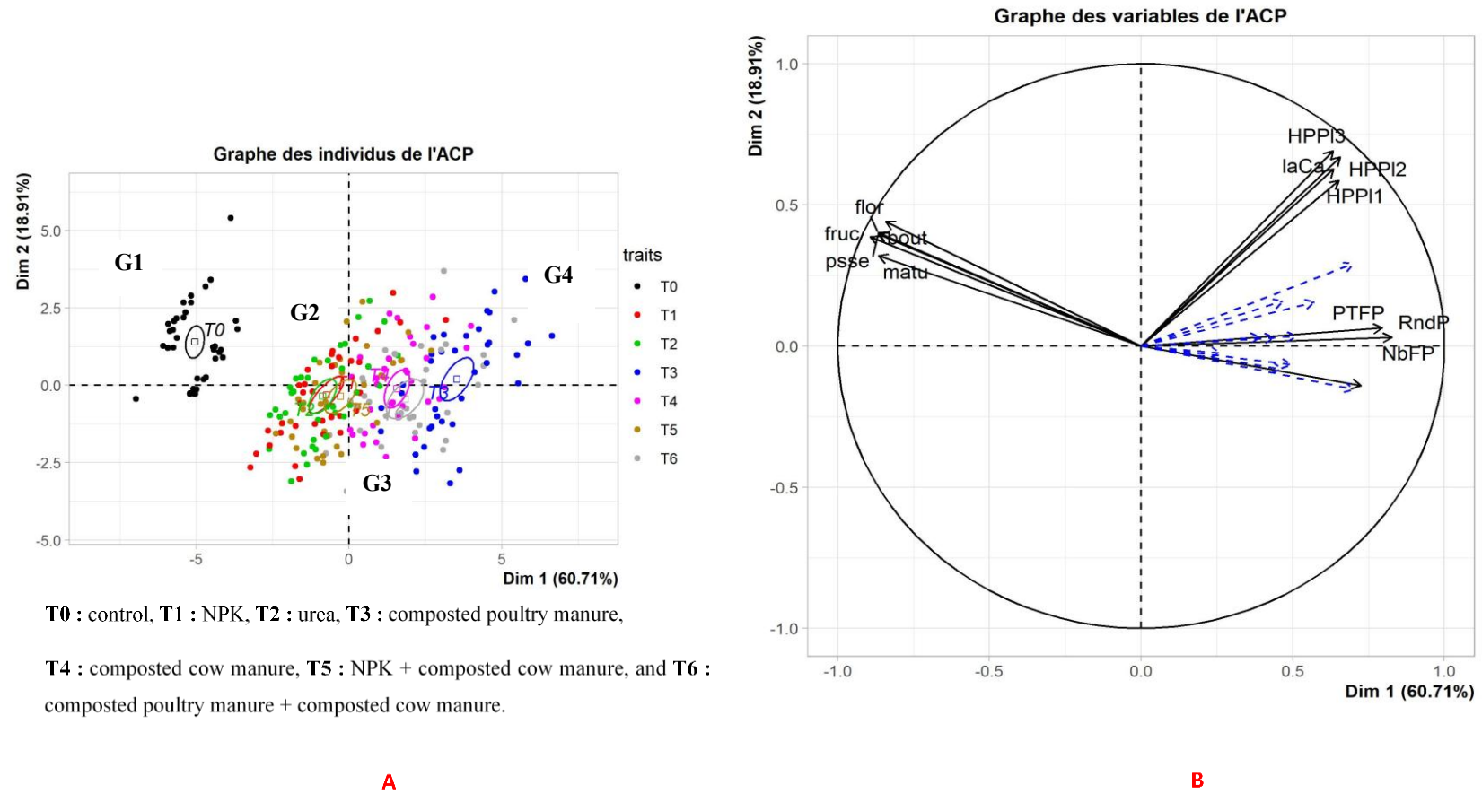
Fig. 5. A : Distribution of individuals according to treatment on the plane formed by the first two PCA axes, and B : Circle of correlations between variables
