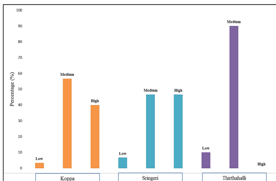
Fig. 5b. Percent distribution of available nitrogen classes of surface soils in the arecanut gardens of selected taluks of Malnad region
