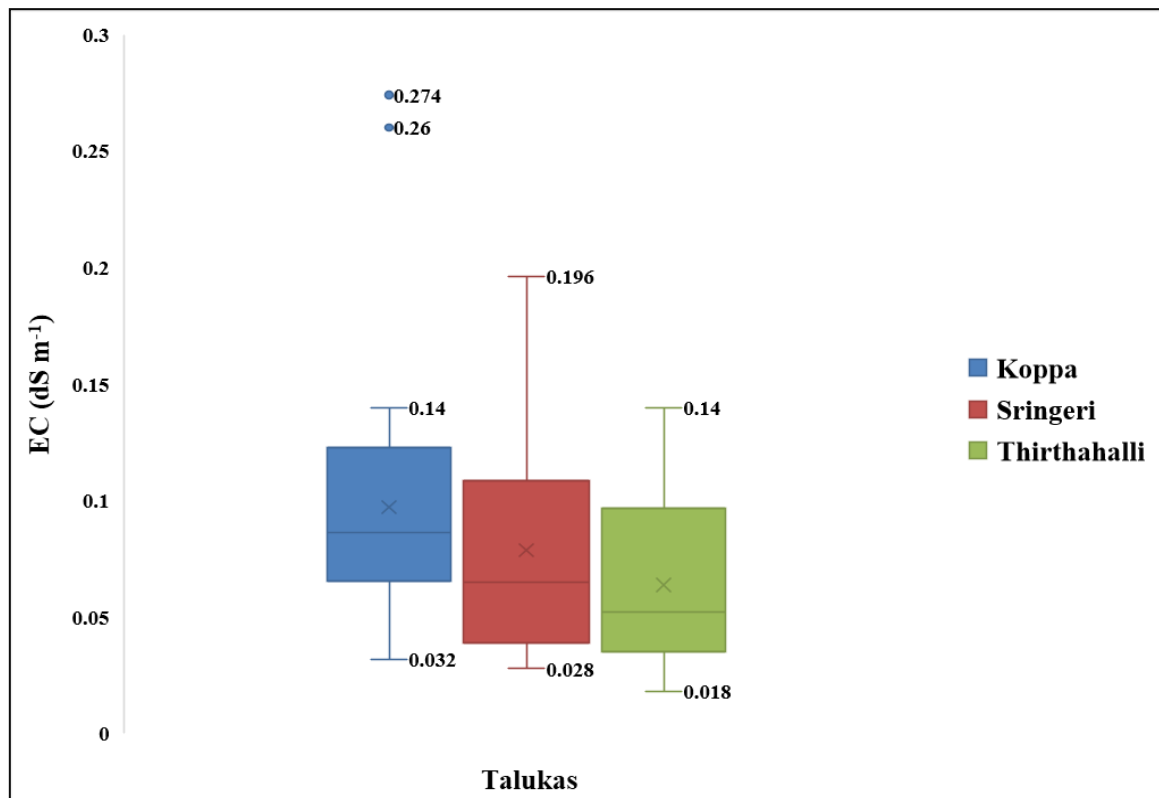
Fig. 3a. Soluble salt content of surface soils in the arecanut gardens of selected taluks of Malnad region
