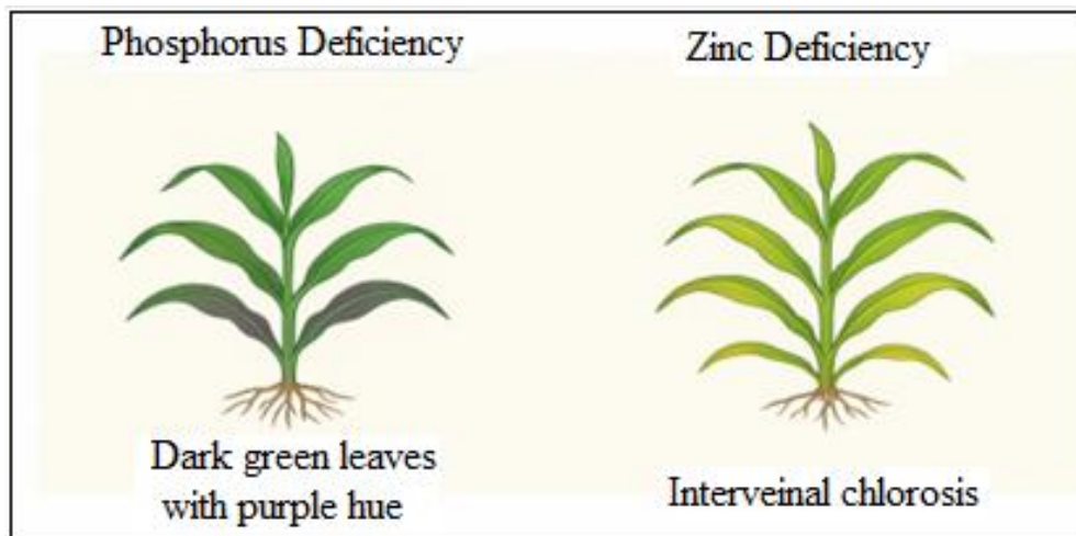
Fig. 4. Phosphorus and zinc deficiency in plants
