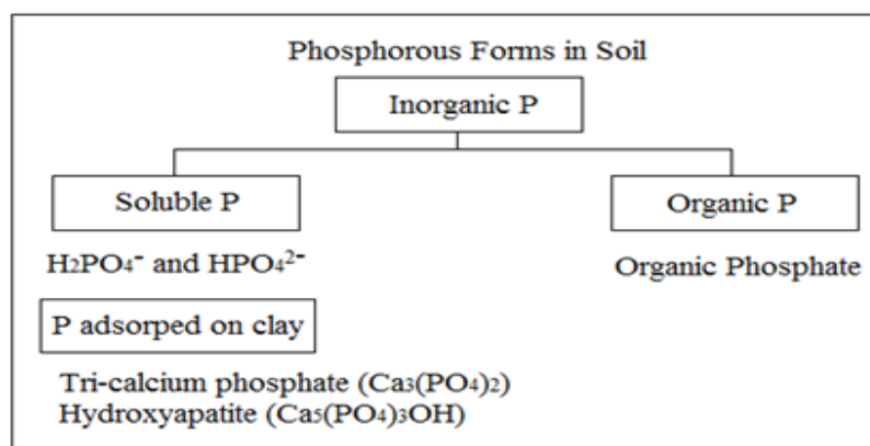
Fig. 1. Phosphorus forms in soil
