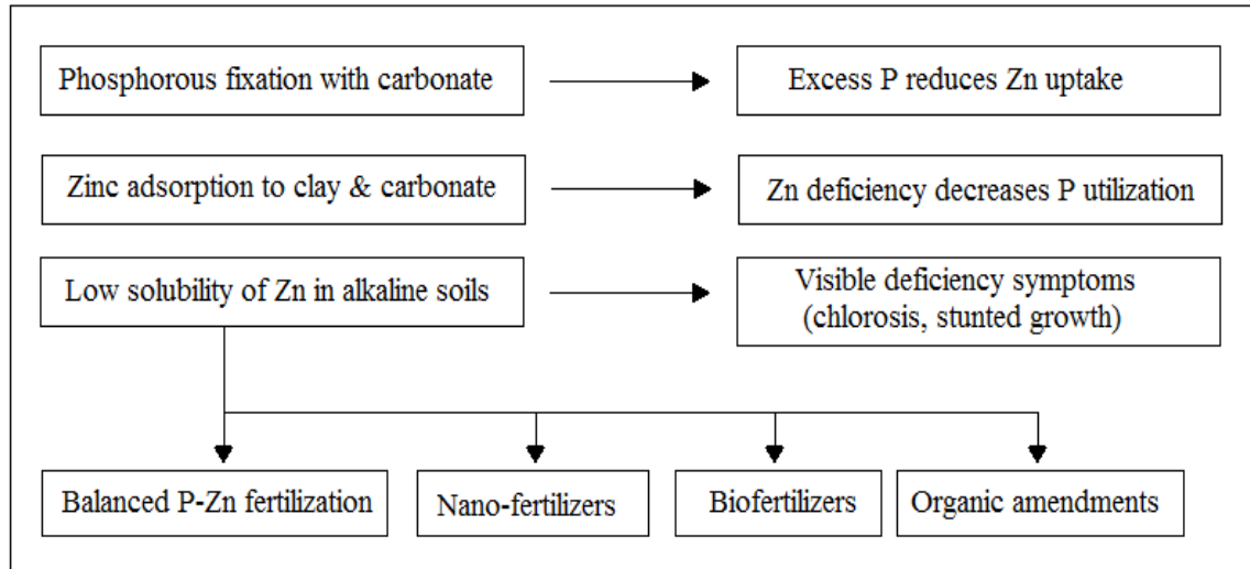
Fig. 3. Interactions of Phosphorus and Zinc in Soil-Plant Systems
