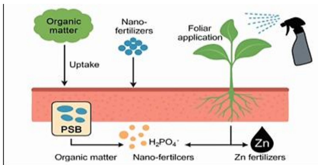
Fig. 5. Mechanisms of increasing P and Zn availability in calcareous soils
