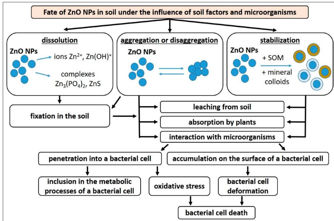
Fig. 2. Key processes determining the fate of ZnO NPs in soil under the influence of soil factors and microorganisms. SOM—soil organic matter
