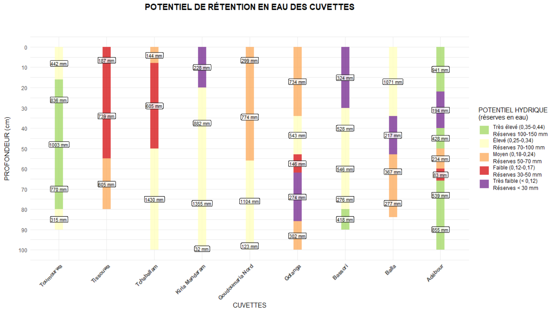
Fig. 3. Water retention capacity of the studied basins
