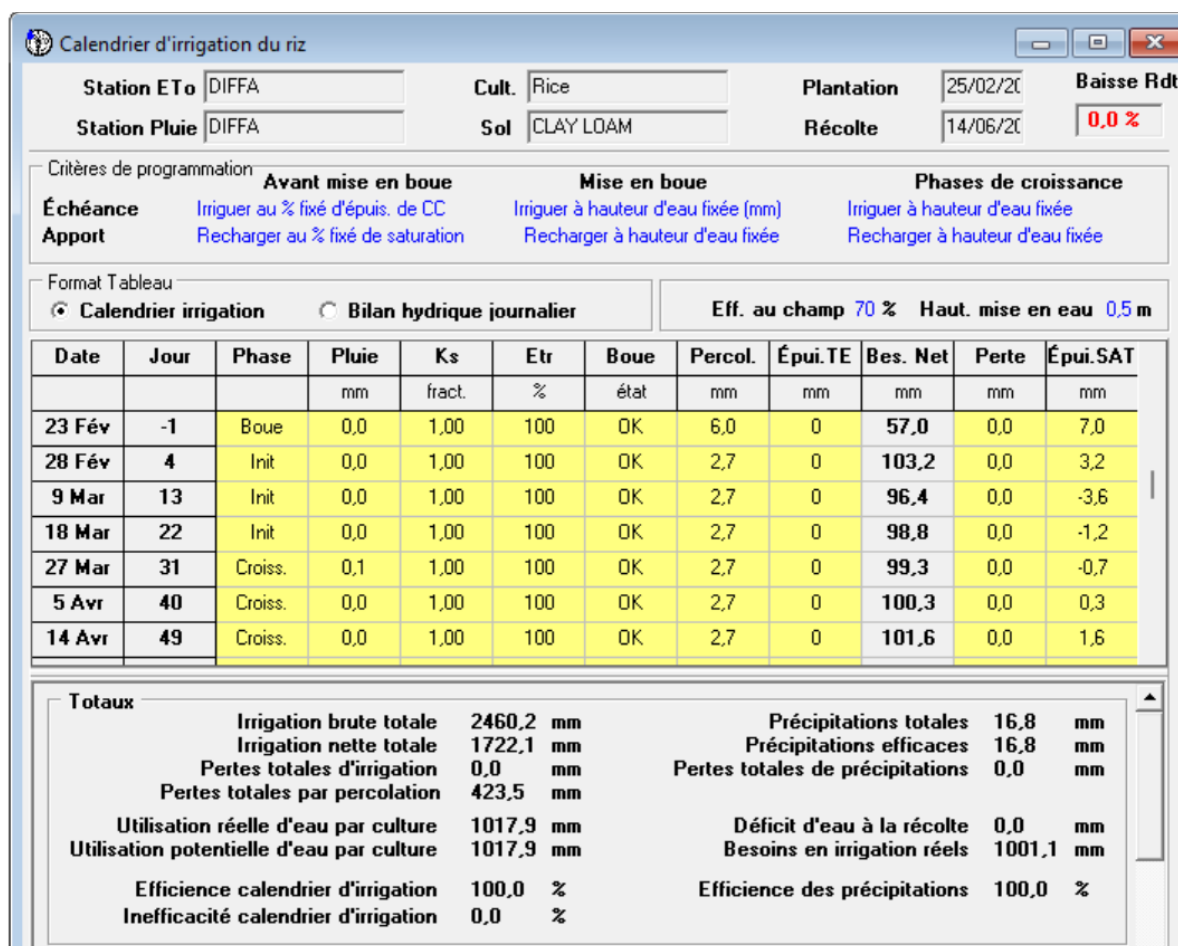
Fig. 9. Results of rice paddy irrigation programming on the site
