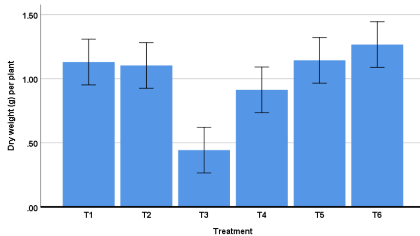
Fig. 3. Effect of different biofertilizers on dry weight (g per plant) at harvest in wheat
