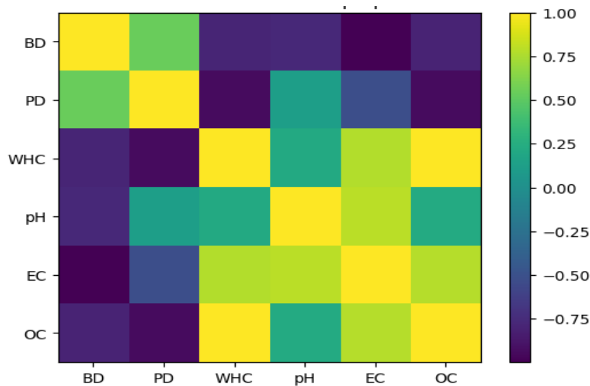
Fig. 2. Correlation matrix of soil properties
