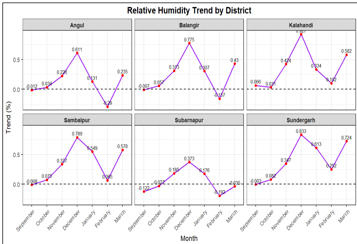
Fig. 10. Graph showing Trend of Relative humidity for the months of growing season of Kharif onion in important onion producing districts of Odisha
