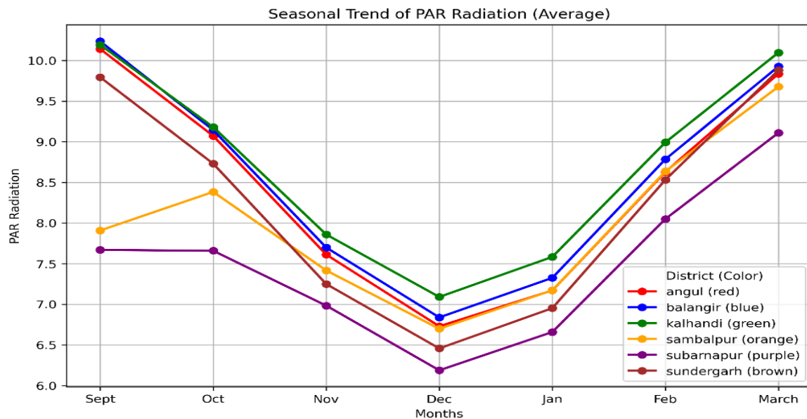
Fig. 4. Graph showing Monthwise variation of PAR ( \text{MJ}/\text{m}^2/\text{day} ) for growing period of onion averaged over the period 1996 to 2023
