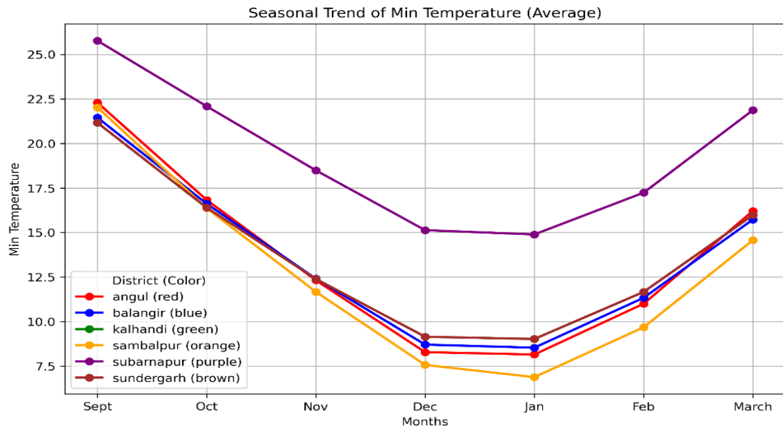
Fig. 3. Graph showing Monthwise variation of Minimum Temperature ( ^{\circ}\text{C} ) for growing period of onion averaged over the period 1996 to 2023
